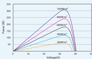
P-V CURVES OF PV MODULE(305W)
